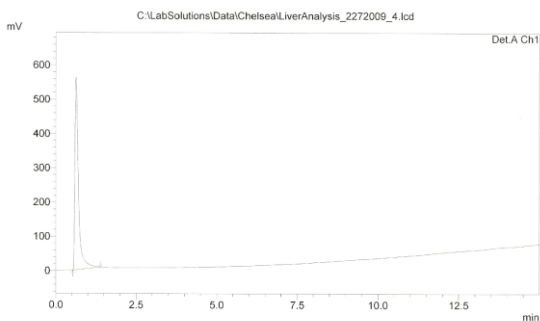
Fig. 4 – Chromatographs of 0.2 M ethanol
